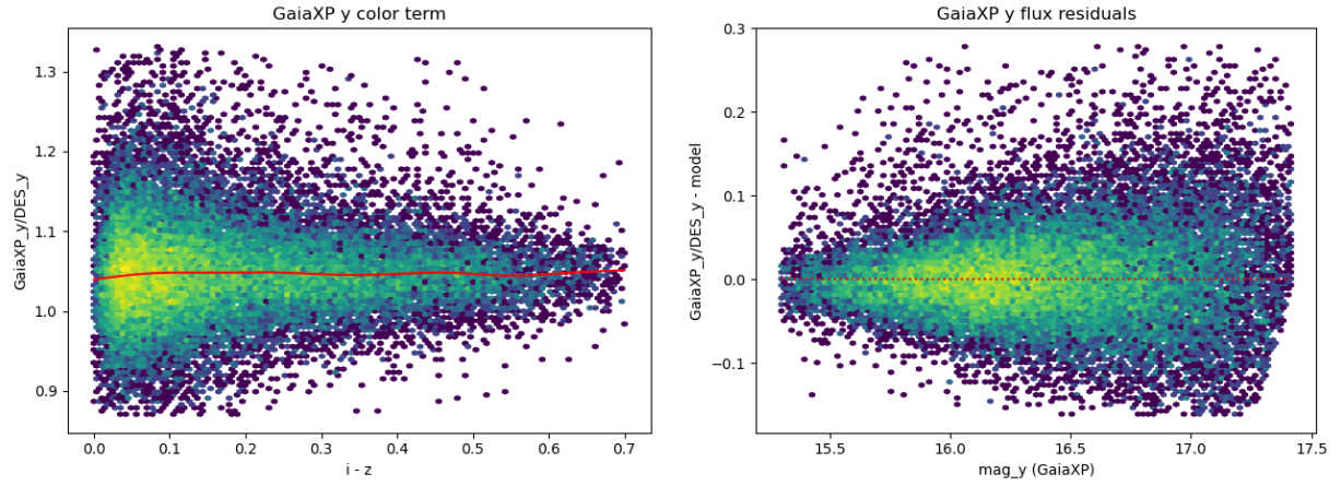
FIGURE 17: Same as figure (13) but for y-band. Note the color transformation is a function of i - z
