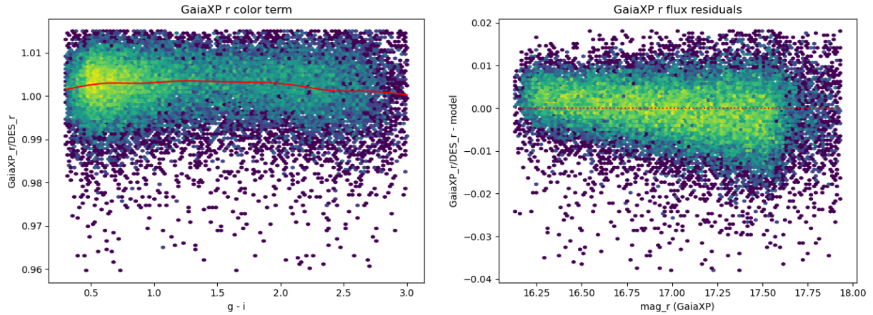
FIGURE 14: Same as figure 13 but for r -band
