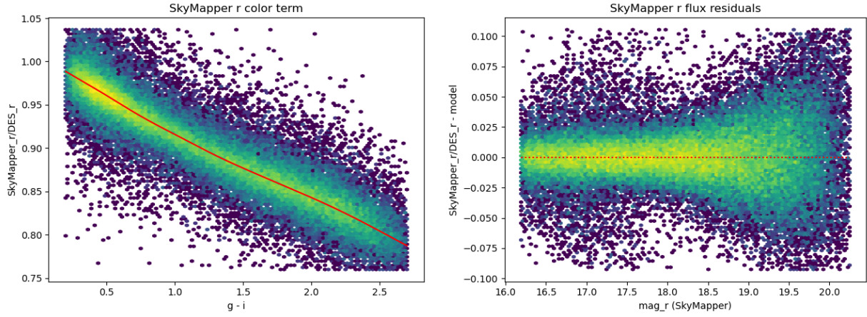
FIGURE 25: Same as figure (24) but for r -band.
