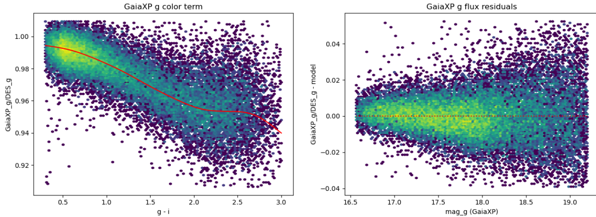
FIGURE 1: Left: The ratio of fluxes between Gaia -XP synthetic photometry and DES for the g -band as a function of g-i color. The red line shows the cubic spline that defines our color transformation. Right: Residuals between Gaia -XP synthetic photometry transformed to DES and DES as a function of magnitude.
