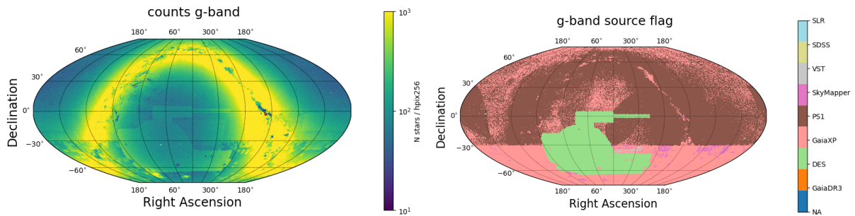
FIGURE 8: Left: Map showing the number of sources with a g -band measurement per NSIDE=256 healpixel. Right: Map showing the median source of objects at each point in the sky for the g band.
