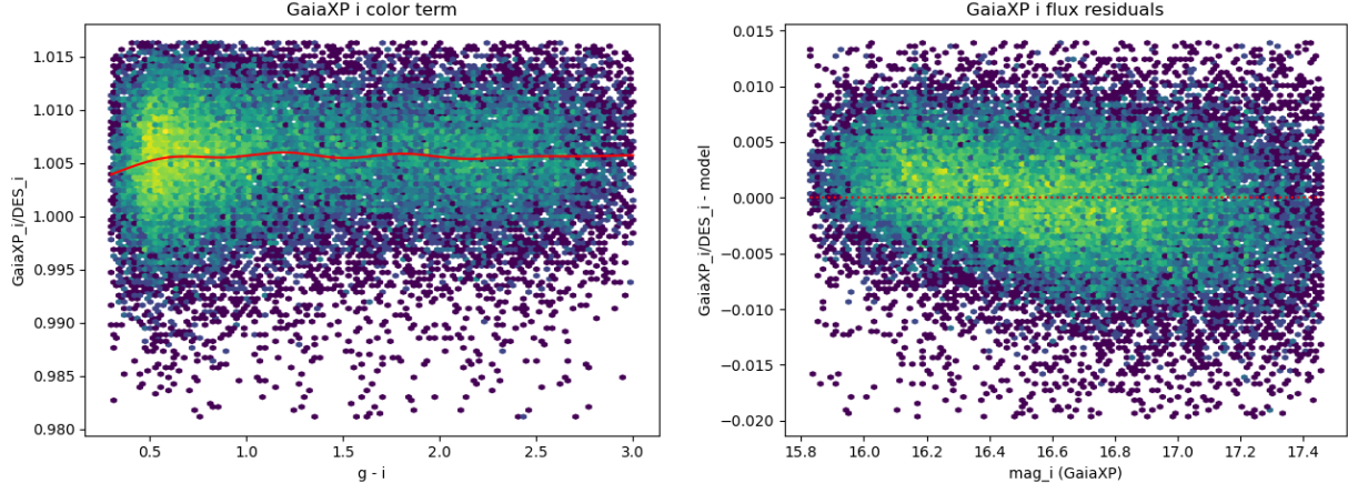
FIGURE 15: Same as figure 13 but for i -band
