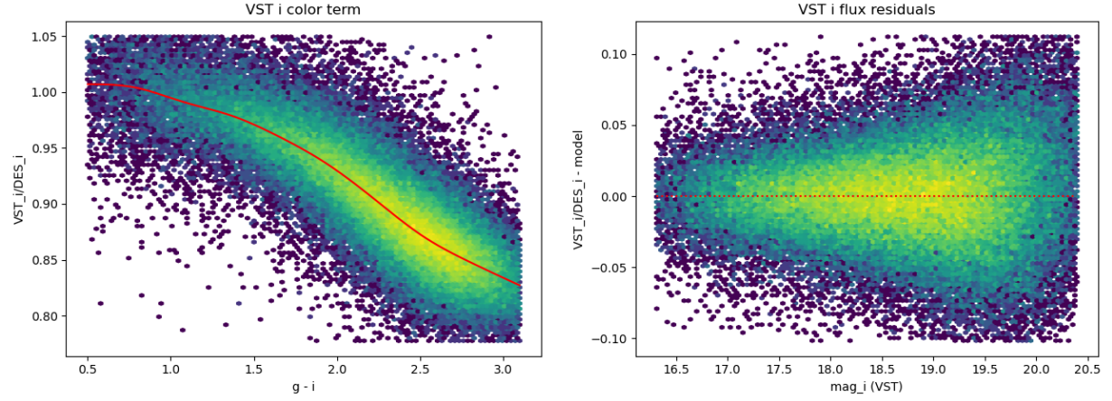
FIGURE 30: Same as figure (28) but for i -band.
