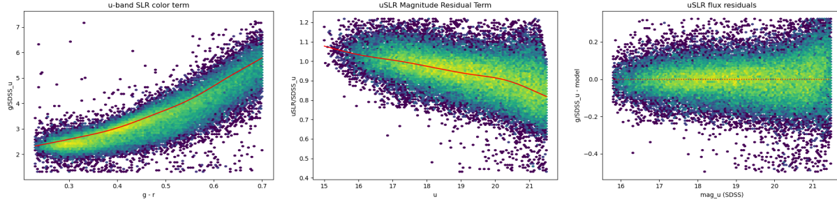
FIGURE 6: Left: The ratio of fluxes between g_{\text{des}} and u_{\text{sdss}} as a function of g_{\text{des}} - r_{\text{des}} color. The red line shows the cubic spline that defines our color transformation. Middle: The ratio of fluxes between u_{\text{slr}} and u_{\text{sdss}} as a function of magnitude demonstrating the need for correcting a magnitude dependence. Right: Residuals between u_{\text{slr}} synthetic photometry and SDSS as a function of magnitude showing a small scatter.
