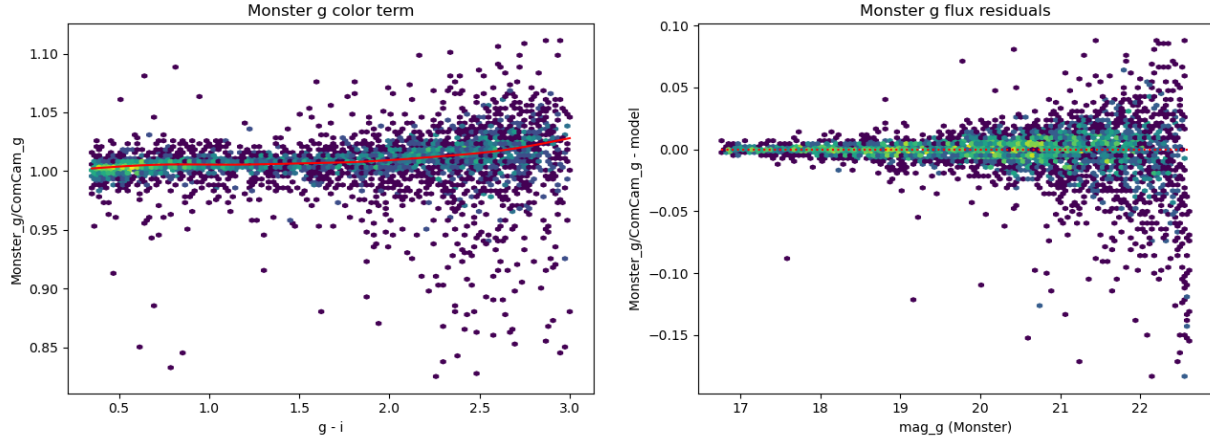
FIGURE 2: Left: The ratio of fluxes between ComCam and Monster(DES) fluxes for the g -band as a function of g-i color. The red line shows the cubic spline that defines our color transformation. Right: Residuals between Monster (DES) photometry and ComCam as a function of magnitude.
