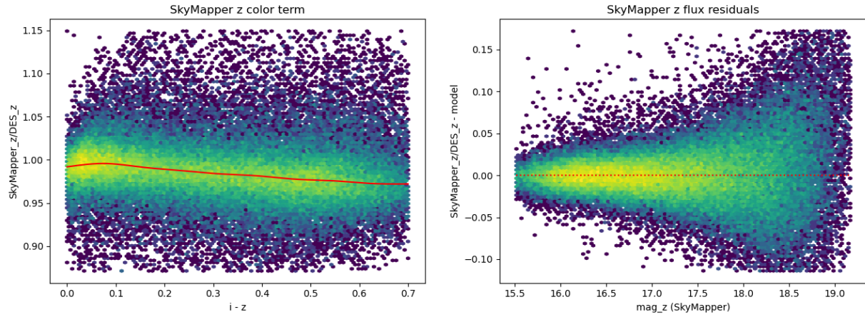
FIGURE 27: Same as figure (24) but for z -band. Note the color transformation is a function of i-z
