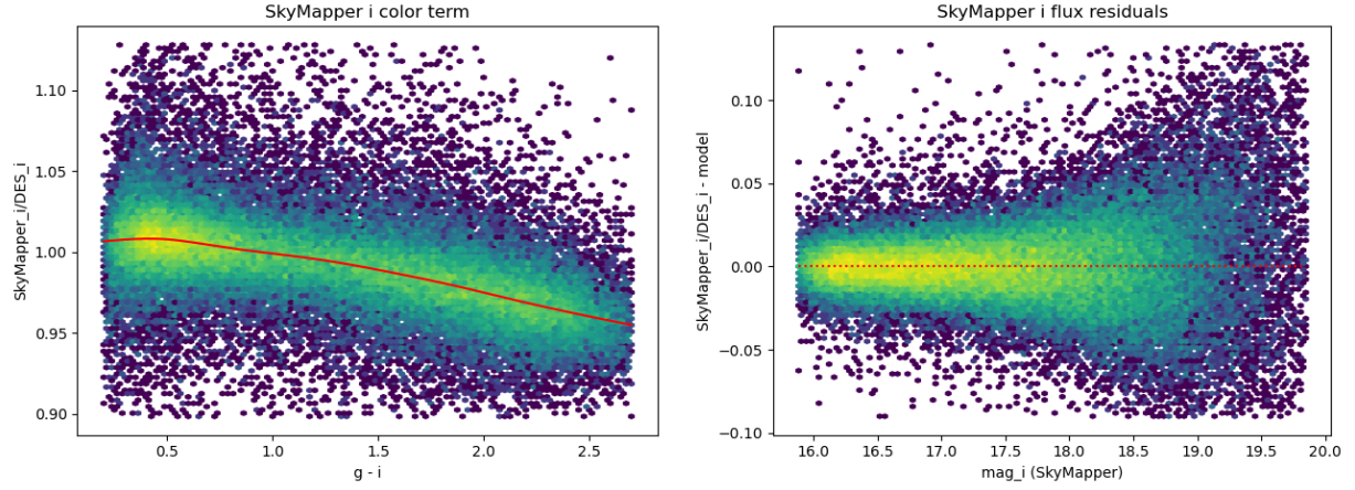
FIGURE 26: Same as figure (24) but for i -band.
