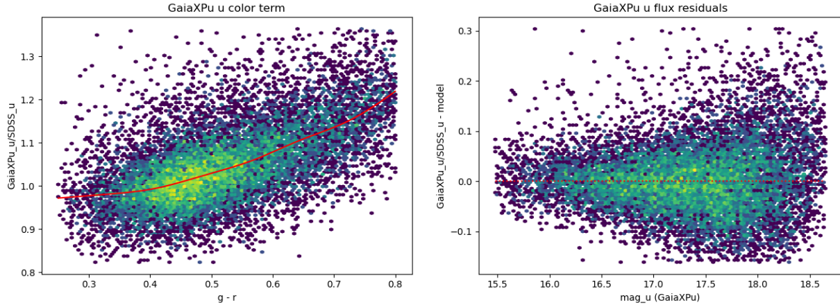
FIGURE 4: Left: The ratio of fluxes between Gaia -XP synthetic photometry and SDSS for the u -band as a function of g-r color. The red line shows the cubic spline that defines our color transformation. Right: Residuals between Gaia -XP synthetic photometry transformed to SDSS and SDSS as a function of magnitude. Note that the Gaia -XP synthetic photometry uses the raw values not the standardized values from Gaia Collaboration et al. (2023a).
