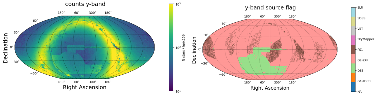
FIGURE 12: Left: Map showing the number of sources with a y-band measurement per n_{\text{side}}=256 healpixel. Right: Map showing the median source of objects at each point in the sky for the y band.
