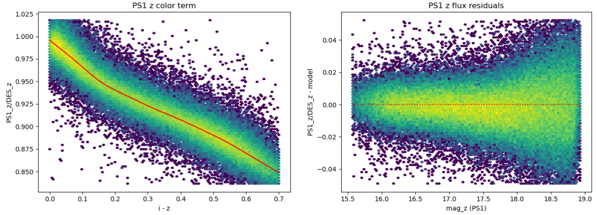
FIGURE 21: Same as figure (18) but for z -band. Note the color transformation is a function of i-z
