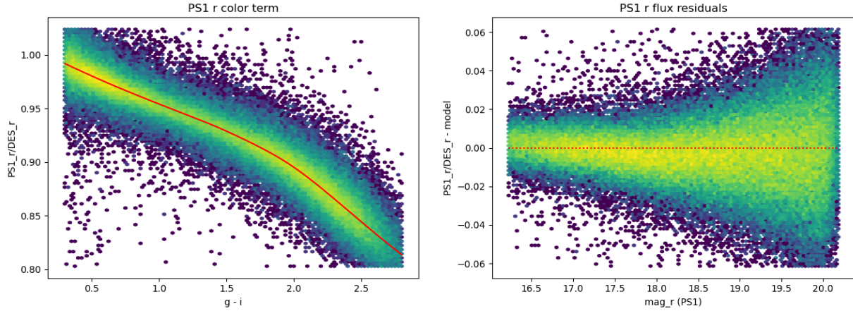
FIGURE 19: Same as figure (18) but for r -band.
