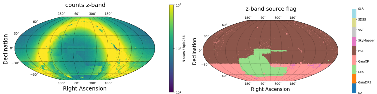
FIGURE 11: Left: Map showing the number of sources with a z -band measurement per n_{\text{side}}=256 healpixel. Right: Map showing the median source of objects at each point in the sky for the z band.
