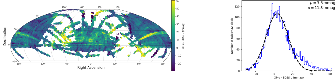
FIGURE 5: Left: Map showing the mean value of u_{\text{GaiaXP}} - u_{\text{SDSS}} as a function of on sky position computed at NSIDE=32 resolution. Right: Histogram of u_{\text{GaiaXP}} - u_{\text{SDSS}} for the high galactic latitude ( |b| > 30 ) regions of the map.
