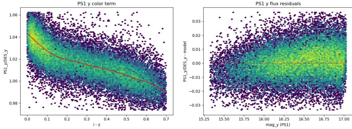
FIGURE 22: Same as figure (18) but for y-band. Note the color transformation is a function of i - z
