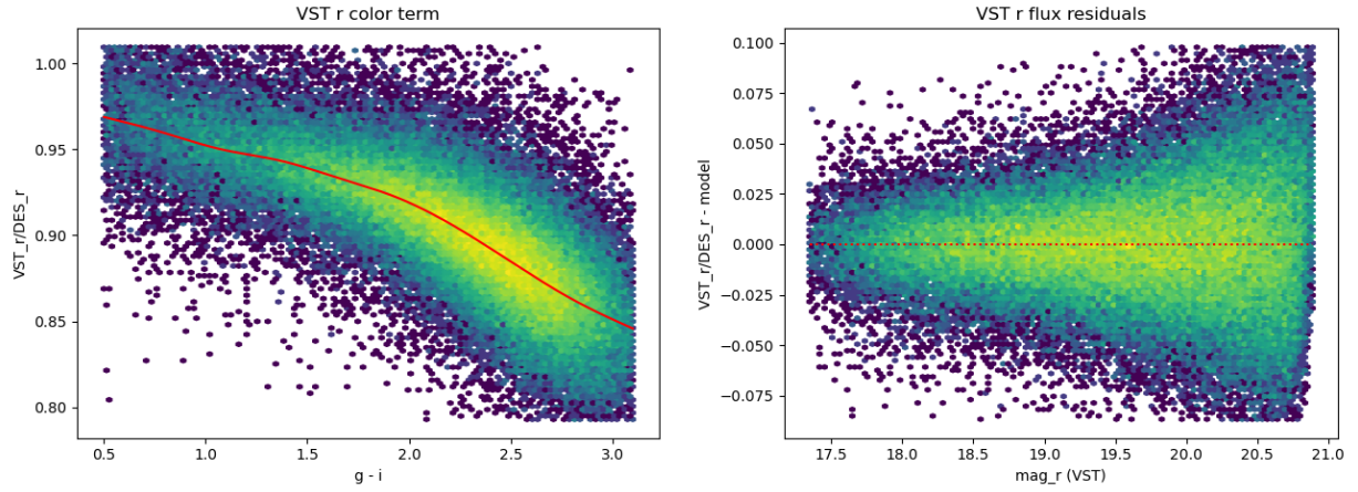
FIGURE 29: Same as figure (28) but for r -band.
