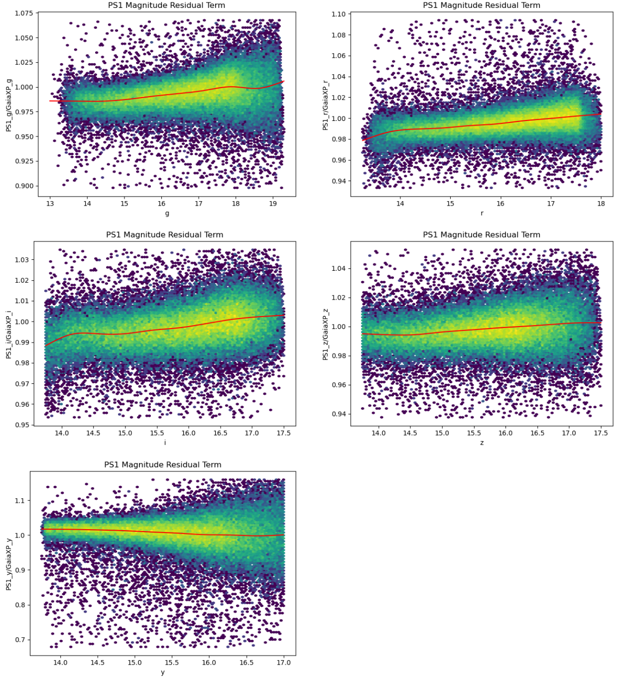
FIGURE 23: Magnitude dependent offsets for PS1 photometry in the DES bandpasses when compared with Gaia -XP synthetic photometry in the DES bandpasses. The offsets are shown as a function of DES magnitude. The red line shows the cubic spline that defines our color transformation.
