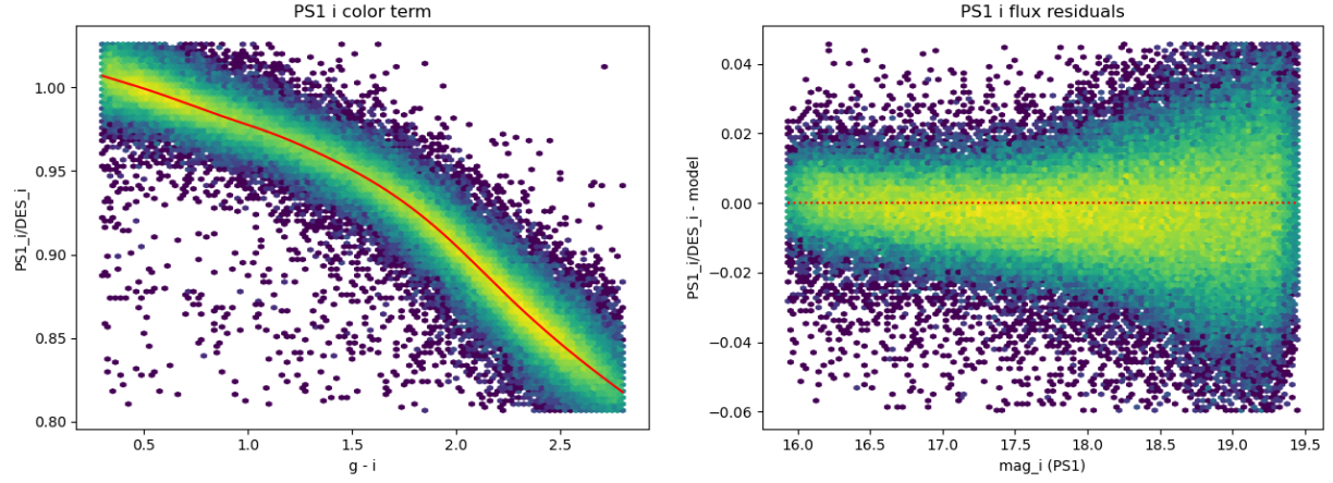
FIGURE 20: Same as figure (18) but for i -band.
