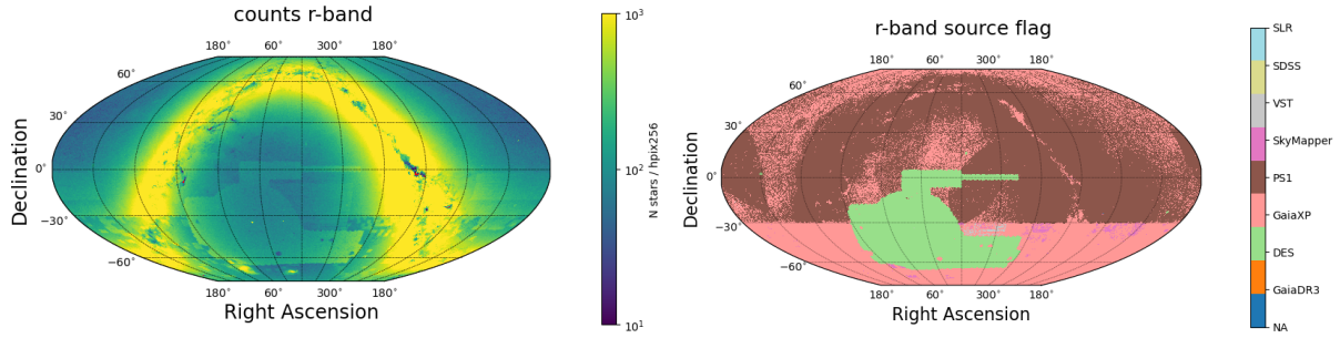
FIGURE 9: Left: Map showing the number of sources with a r -band measurement per n_{\text{side}}=256 healpixel. Right: Map showing the median source of objects at each point in the sky for the r band.
