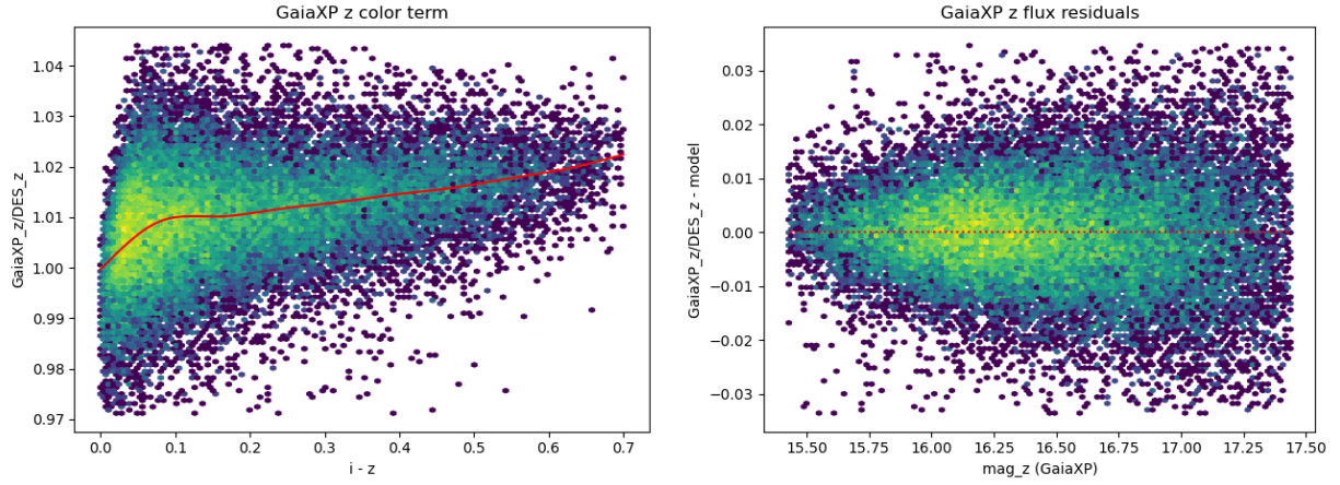
FIGURE 16: Same as figure 13 but for z -band. Note the color transformation is a function of i-z
