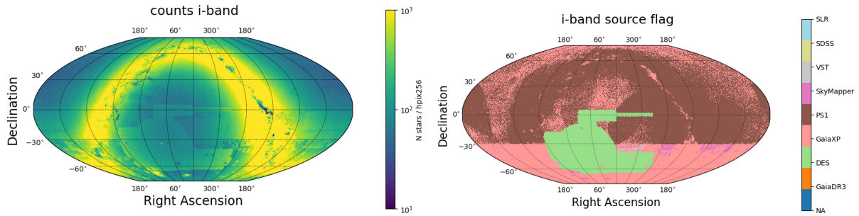
FIGURE 10: Left: Map showing the number of sources with a i -band measurement per n_{\text{side}}=256 healpixel. Right: Map showing the median source of objects at each point in the sky for the i band.
