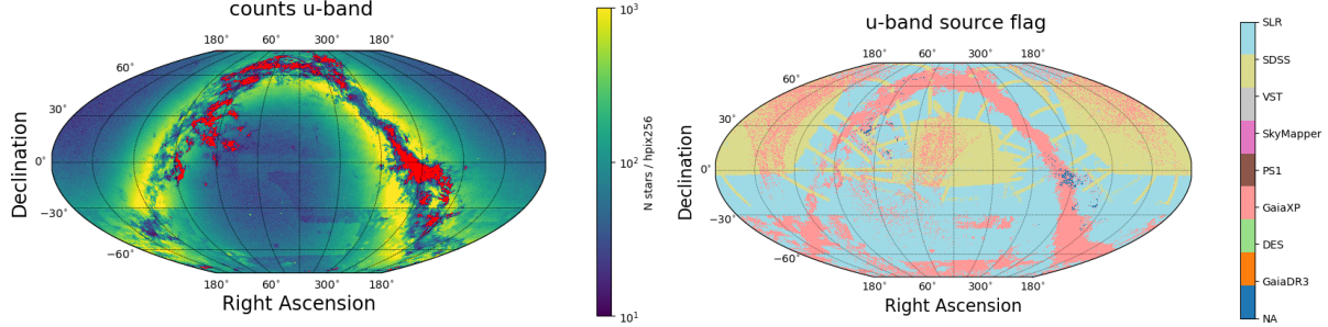
FIGURE 3: Left: Map showing the number of sources with a u -band measurement per NSIDE=256 healpixel. The red regions show the areas with fewer than 10 sources per healpixel. For the u -band, the median source density is \sim 70 sources per healpixel. Of the region accessible by Rubin Observatory ( \delta < 30 ) only \sim 750 sq deg (2.5% of the sky, at very low-galactic latitudes) has a source density lower than 10 sources per healpixel. Right: Map showing the median source of objects at each point in the sky for the u band.
