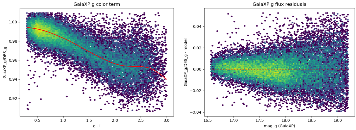
FIGURE 13: Left: The ratio of fluxes between Gaia -XP synthetic photometry and DES for the g -band as a function of g-i color. The red line shows the cubic spline that defines our color transformation. Right: Residuals between Gaia -XP synthetic photometry transformed to DES and DES as a function of magnitude.
