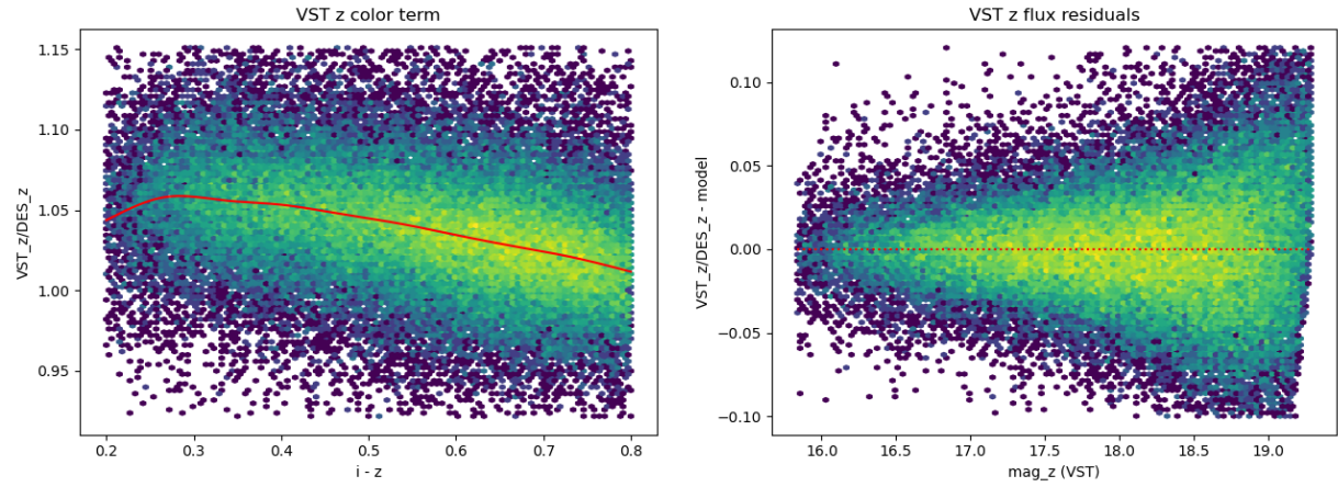
FIGURE 31: Same as figure (28) but for z -band. Note the color transformation is a function of i-z
