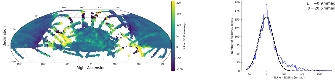
FIGURE 7: Left: A map showing the mean value of u_{\text{slr}} - u_{\text{sdss}} as a function of on sky position computed at NSIDE=32 resolution. Right: Histogram of u_{\text{slr}} - u_{\text{sdss}} for the high galactic latitude ( |b| > 30 ) regions of the map.
